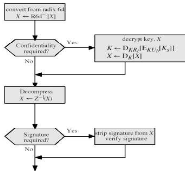
(b) Generic Reception Diagram (to B)
