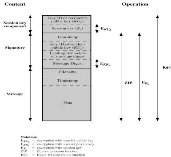
Figure 4: General format of PGP message (from A to B).
