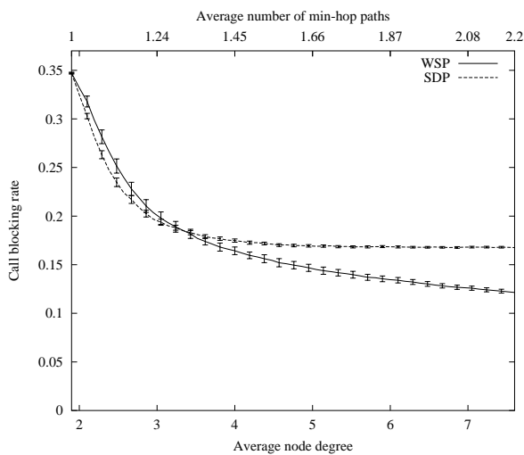
Fig. 7. Call blocking probability of WSP and SDP under increasing node degree, \rho = 0.8 , hd = 40sec
