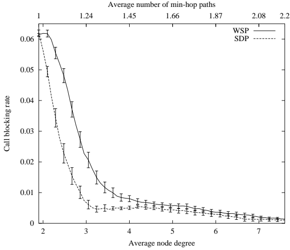
Fig. 4. Call blocking probability of WSP and SDP under increasing node degree, \rho = 0.3 , hd = 40sec
