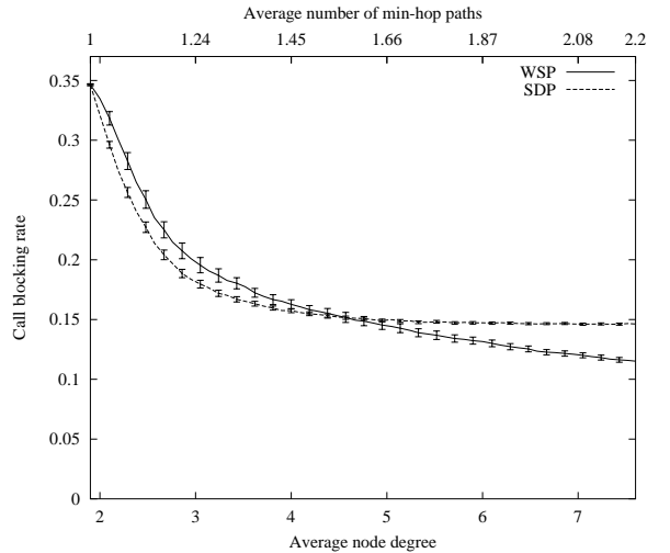
Fig. 6. Call blocking probability of WSP and SDP under increasing node degree, \rho = 0.8 , hd = 20sec
