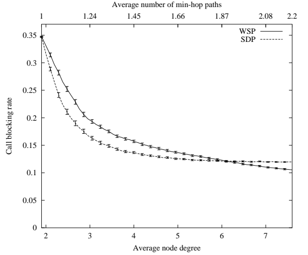
Fig. 5. Call blocking probability of WSP and SDP under increasing node degree, \rho = 0.8 , hd = 1sec
