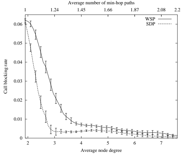
Fig. 3. Call blocking probability of WSP and SDP under increasing node degree, \rho = 0.3 , hd = 1sec
