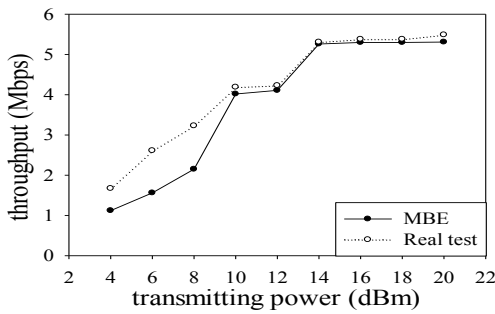
Fig. 8 Transmitted power effect on throughput
