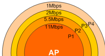
Fig. 9 Theoretical wireless link capacity for IEEE 802.11b
