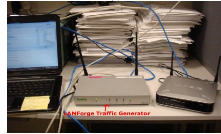
Fig. 5 (a) Test bed topology (b) Real test bed including traffic generator and 802.11AP
