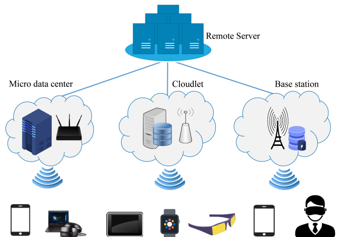
Fig. 12: Architecture of mobile edge-assisted streaming of 360° video.
