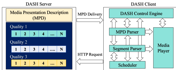
Fig. 4: MPEG-DASH client-server model.
