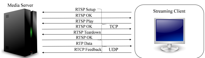
Fig. 2: Traditional RTSP streaming system.
