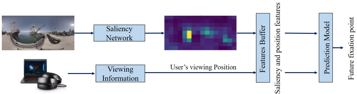
Fig. 14: Saliency and viewing position based fixation prediction network.
