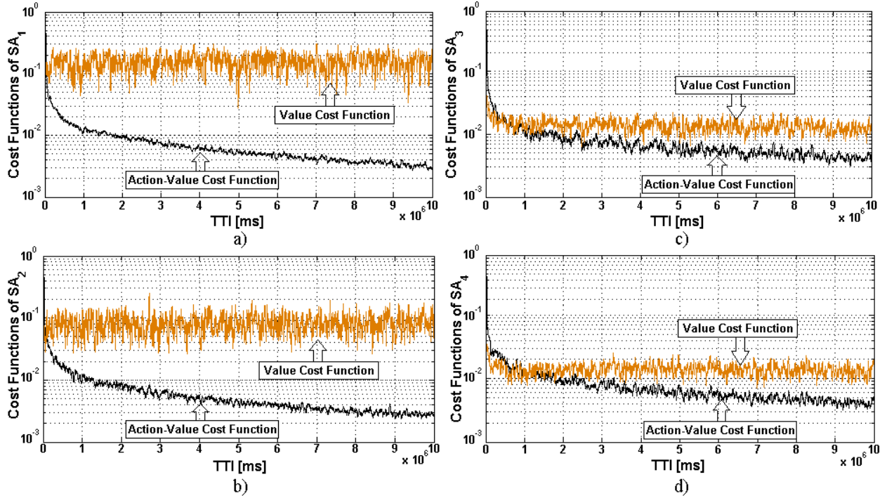
Fig. 8: Training stage of the slave controller a) cost function of slave agent 1 ( video_1 ); b) cost function of slave agent 2 ( video_2 ); c) cost function of slave agent 3 ( video_3 ); d) cost function of slave agent 4 ( video_4 ).
