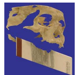
Texture Mapping
