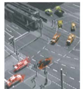
Feature Tracking
