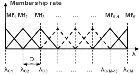
Fig. 6. Triangle shaped membership functions.
