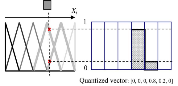
Fig. 10. The fuzzy-based vector quantization procedure. This diagram illustrates the calculation of the quantized vectors when six fuzzy sets are employed to sample the hyperspectral domain.
