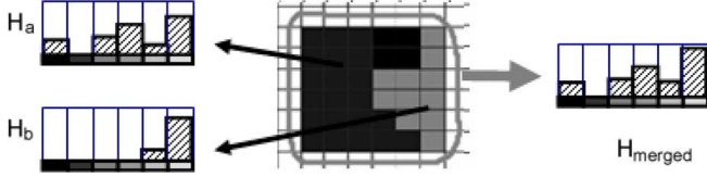
Fig. 14. Histograms of the two candidate regions ( H_a , H_b ) and the histogram of the merged region ( H_{merged} ).
